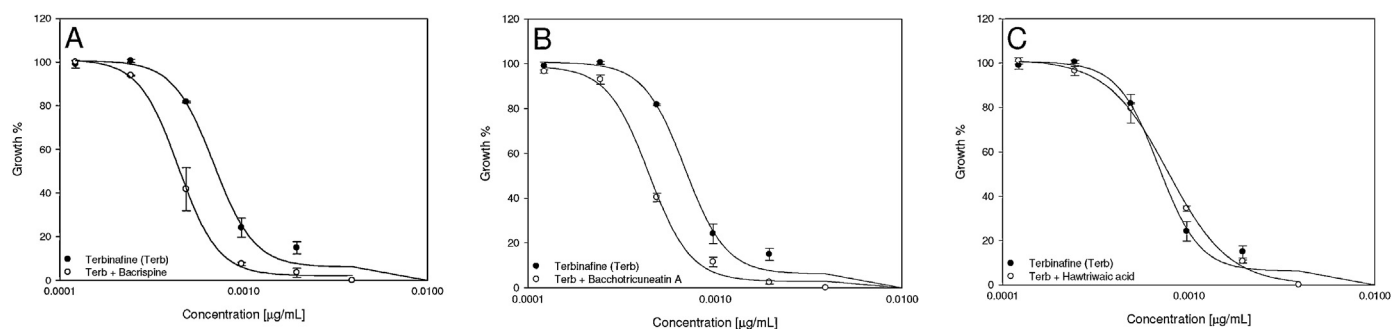
Fig. 8. Dose–response curves of the antifungal drug terbinafine in combination with a fixed amount (31.25 \mu\text{g}/\text{ml} ) of each ent-clerodane bacrispine 5 (A), bacchotricuneatin A 6 (B) and hawtriwaic acid 7 (C), detected in Baccharis extracts.
